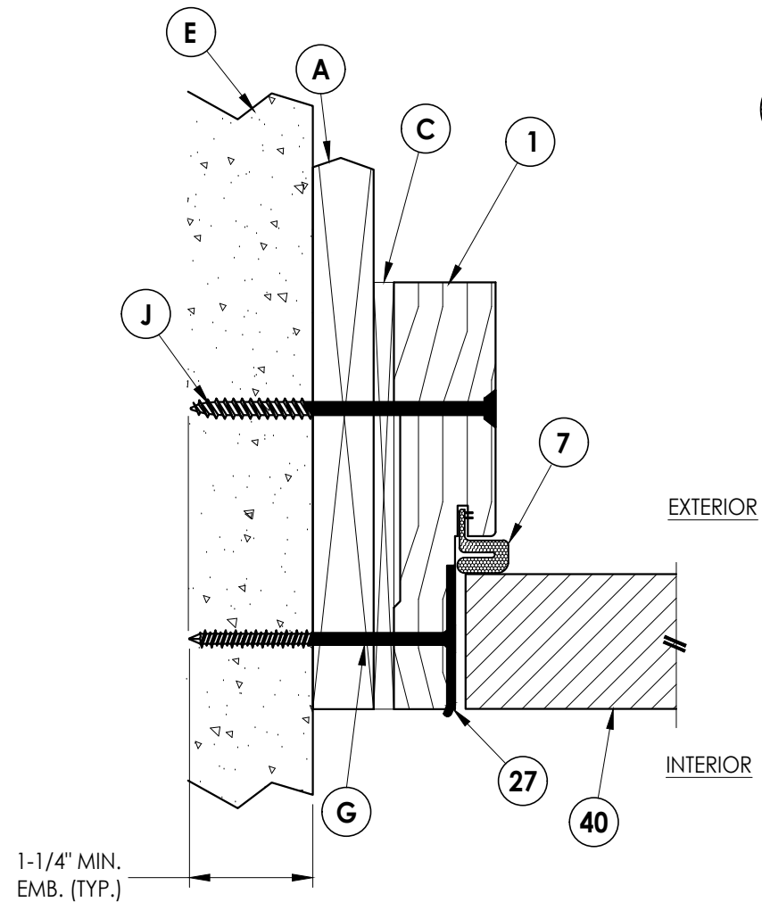
1 4 HORIZONTAL CROSS SECTION Shown w/ 1X sub-buck Inswing shown (Outswing similar)
