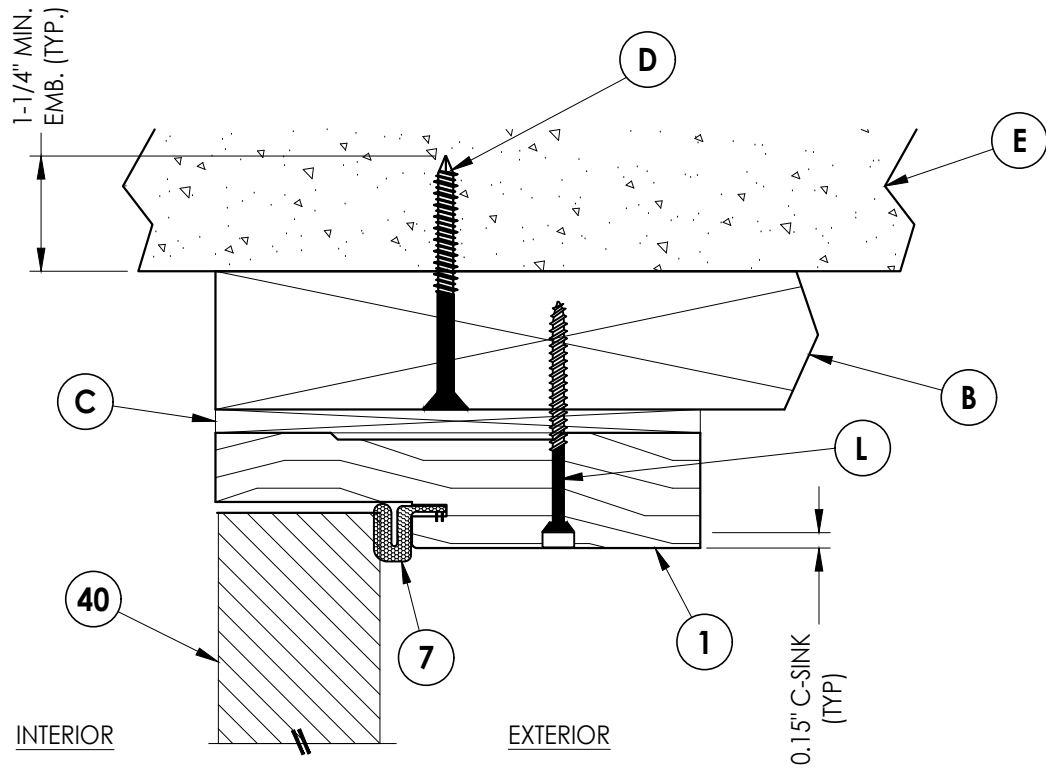
3 VERTICAL CROSS SECTION 3 Shown w/ 2X Buck Inswing shown (Outswing similar)
