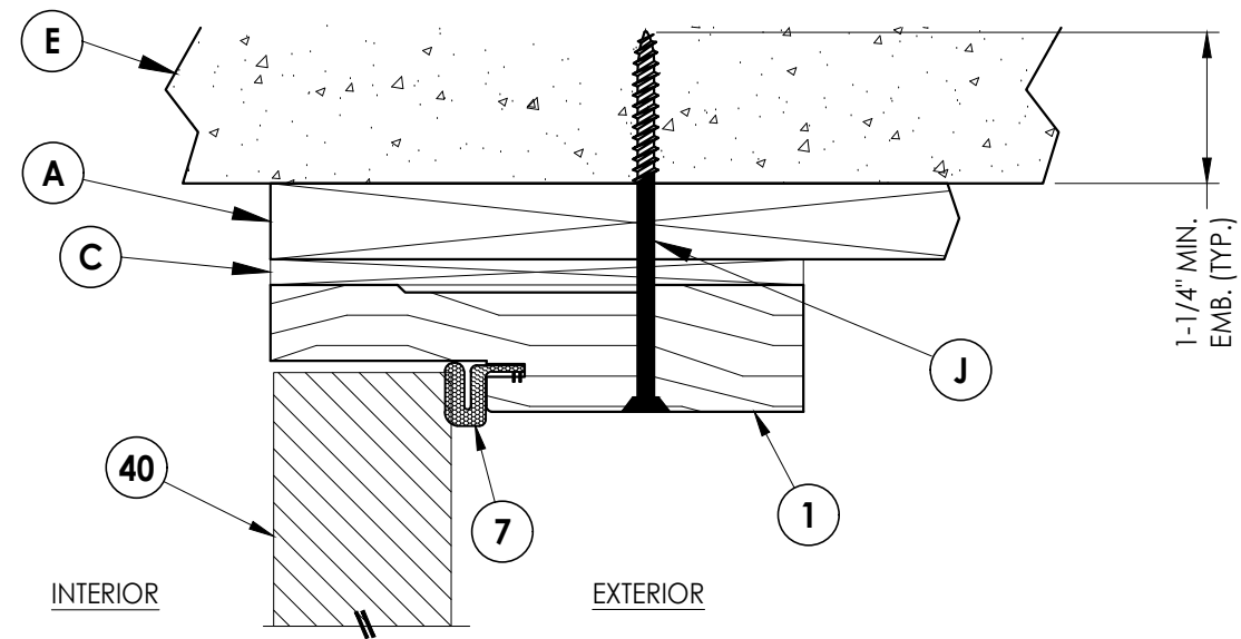
3 VERTICAL CROSS SECTION 4 Shown w/ 1X sub-buck Inswing shown (Outswing similar)
