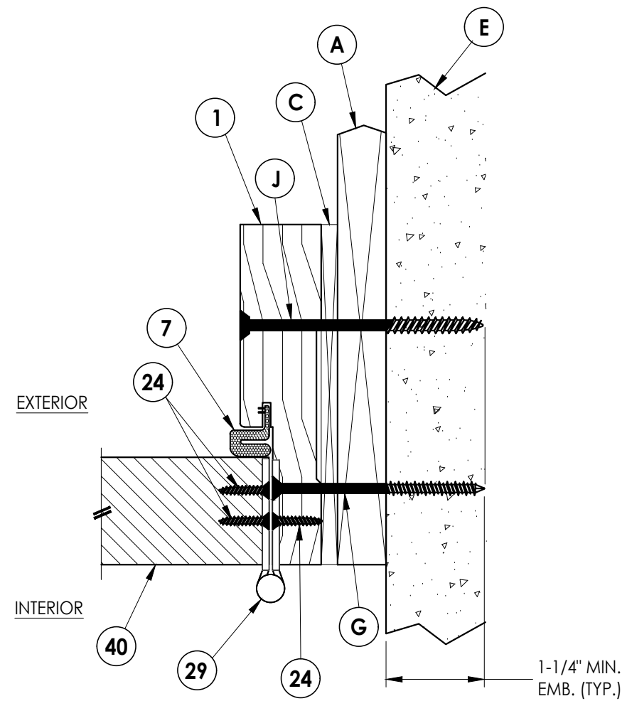
2 HORIZONTAL CROSS SECTION 4 Shown w/ 1X sub-buck Inswing shown (Outswing similar)
